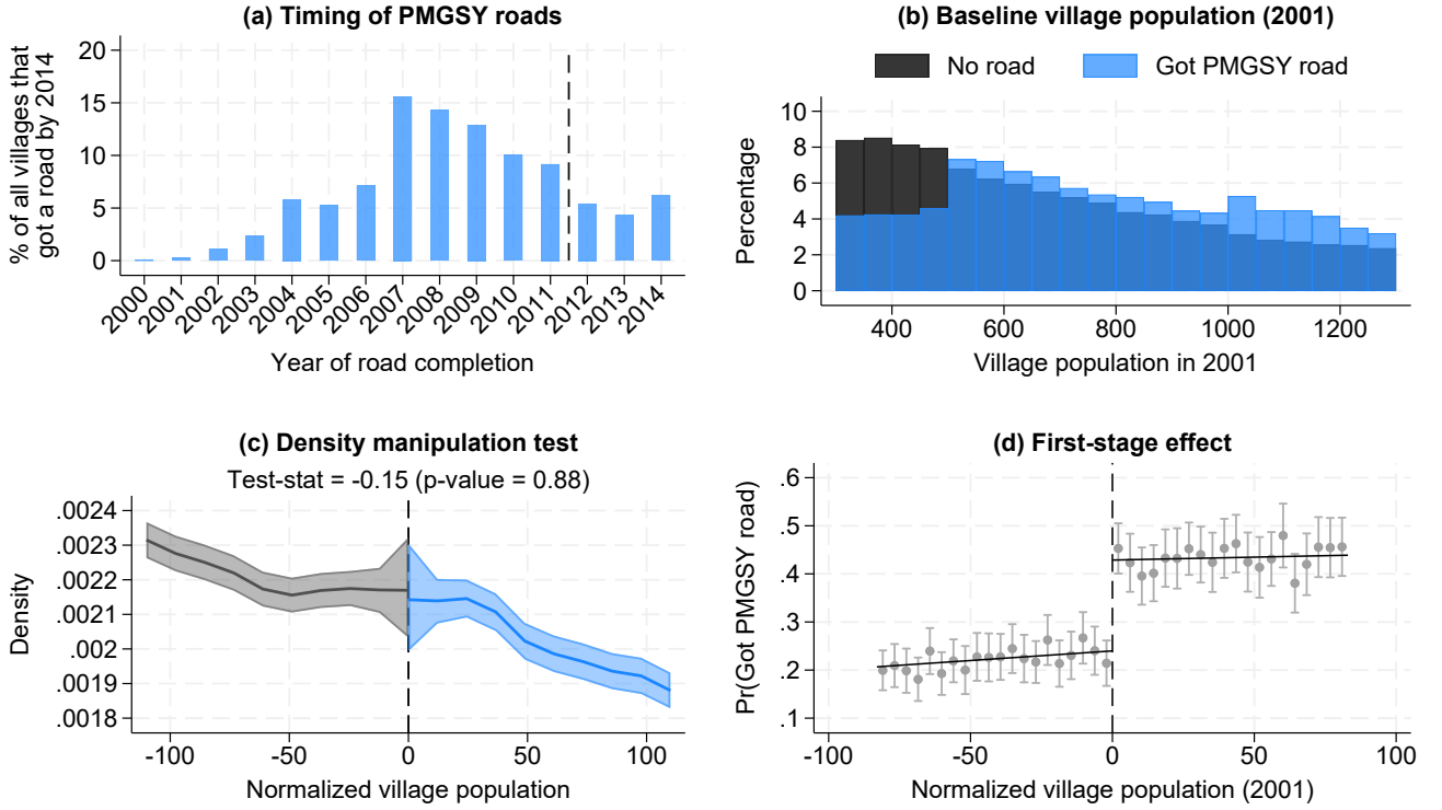
Figure 3: Validating the identification strategy
