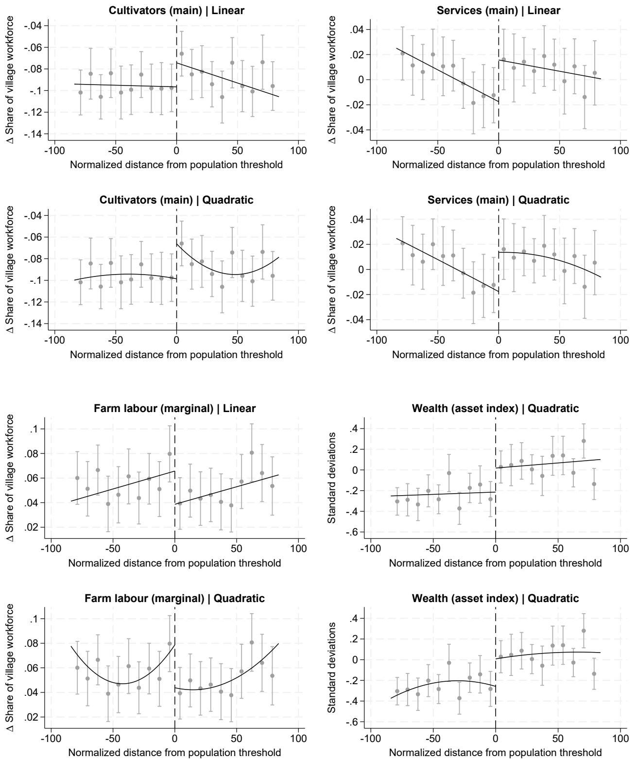
Figure A4: Robustness to order of local polynomial (linear versus quadratic)
